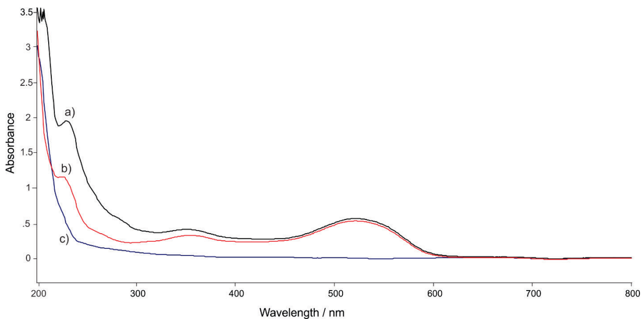
Figure S1. UV/VIS spectrum from: a) Oil red loaded liposomes (OL), b) Oil red solution 0.01 mg/ml (O) and c) ultrafiltration eluate from Oil red loaded liposomes
