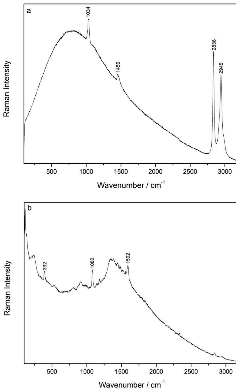
Figure S1. Raman spectra of 4-ATP stock solution, c(4\text{-ATP}) = 2 \times 10^{-3} mol/L. Excitation at a) 532 nm and b) 785 nm.
