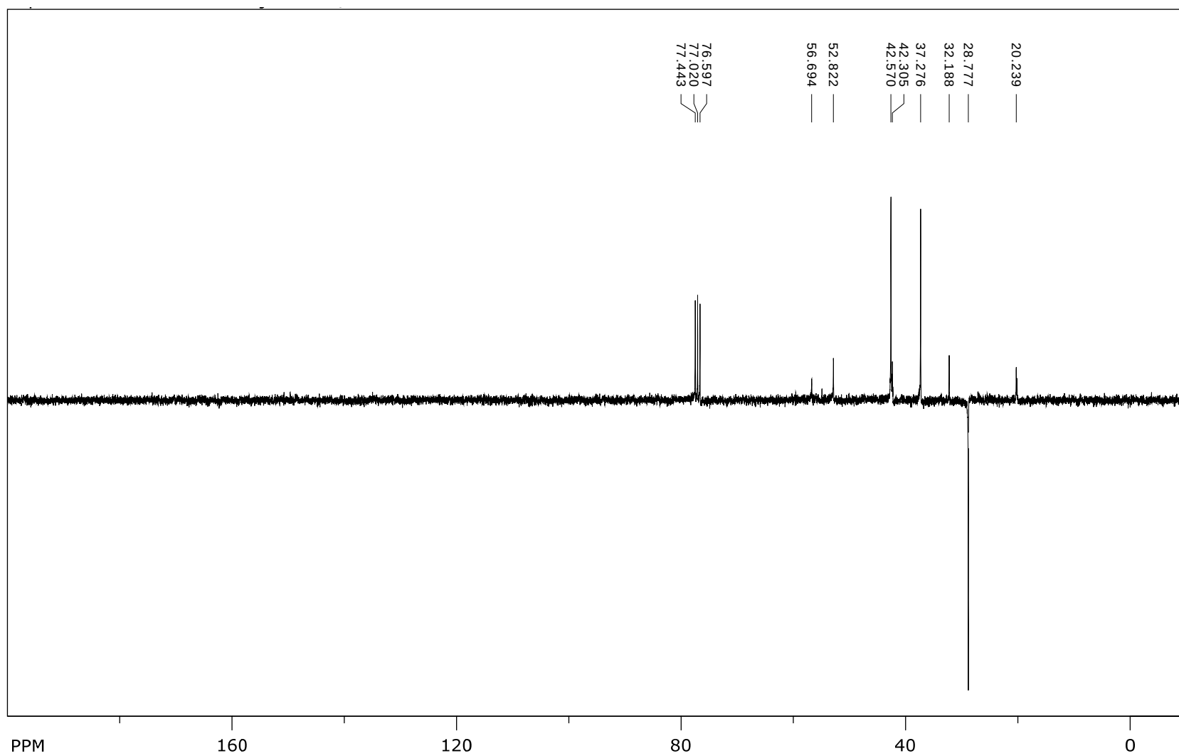
Figure S6. 13 C NMR (75 MHz, CDCl 3 ) spectrum of compound 3 .
