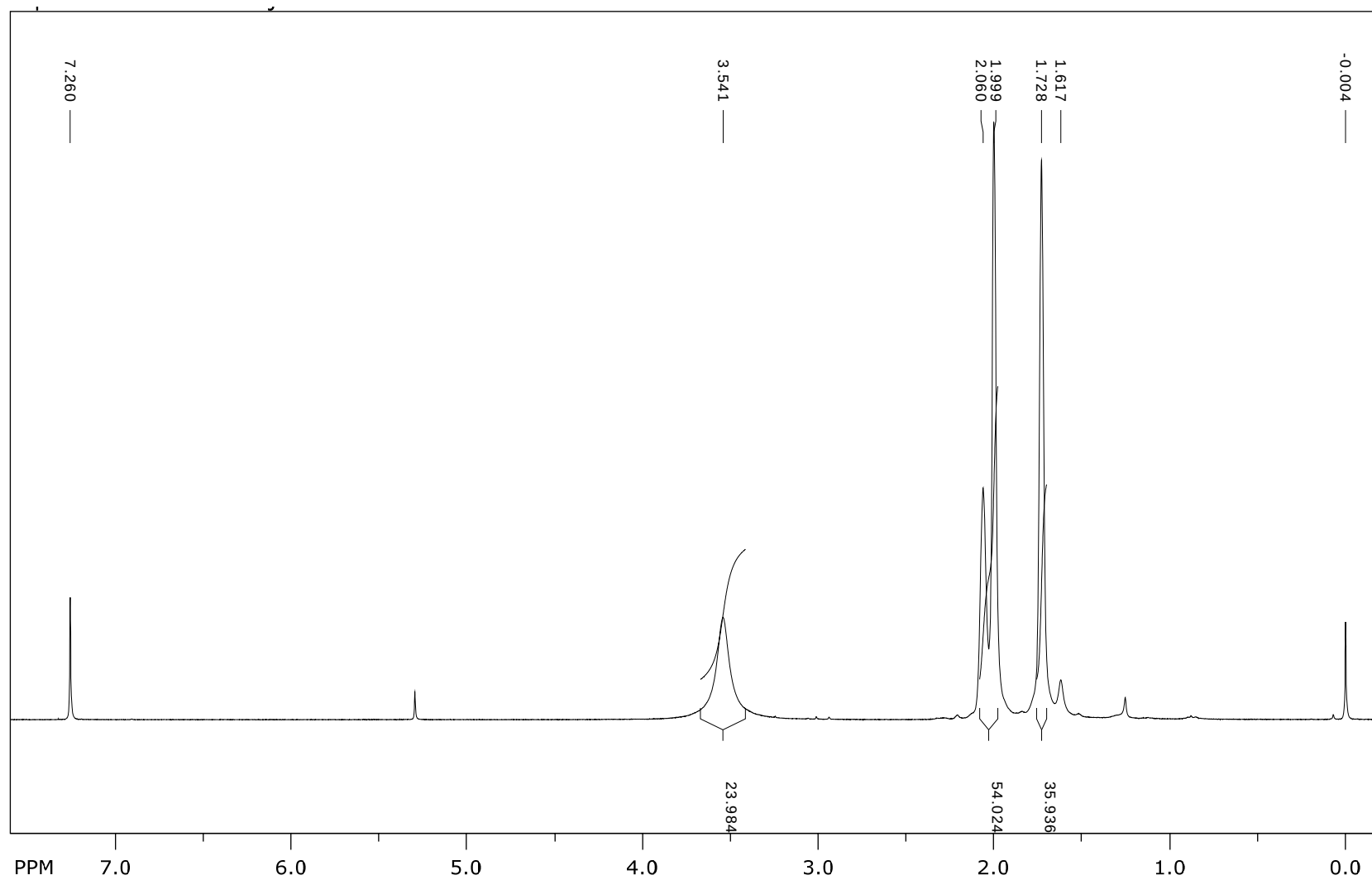
Figure S7. 1 H NMR (300 MHz, CDCl 3 ) spectrum of compound 4.
