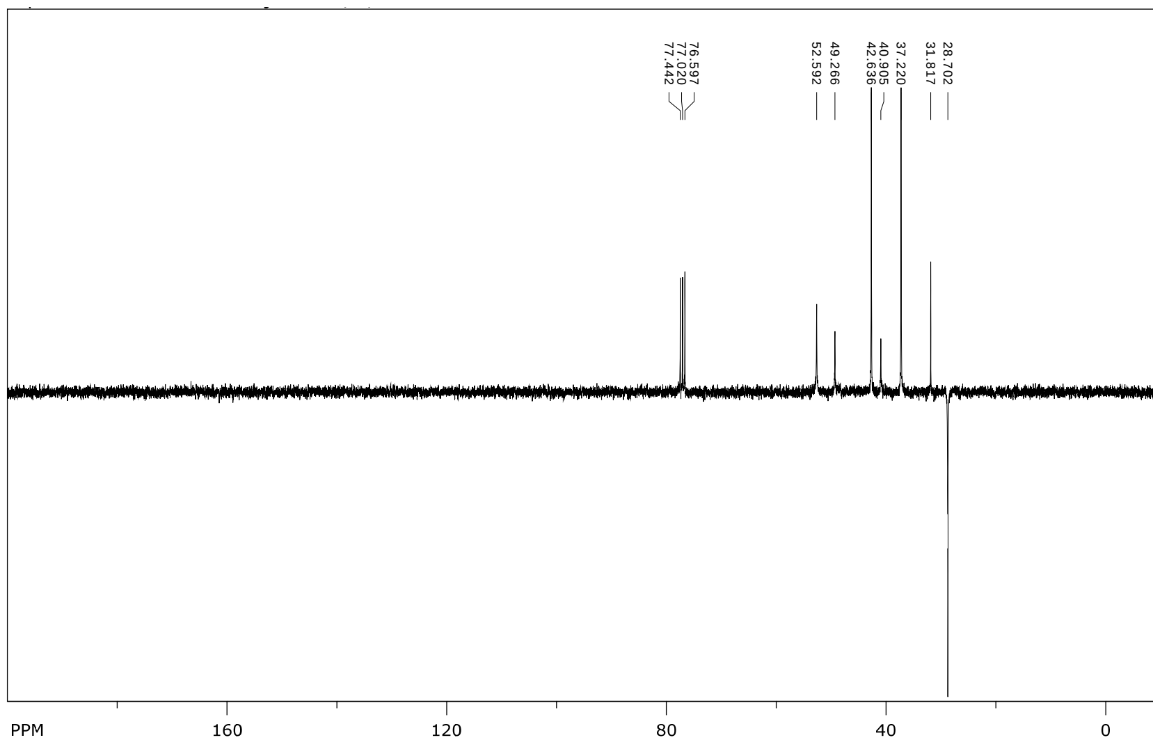
Figure S4. 13 C NMR (75 MHz, CDCl 3 ) spectrum of compound 2 .
