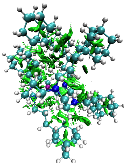
Figure S14. NCI plots for Na + complexes of compounds 1–3 . Attractive non-covalent interactions are depicted in green.
