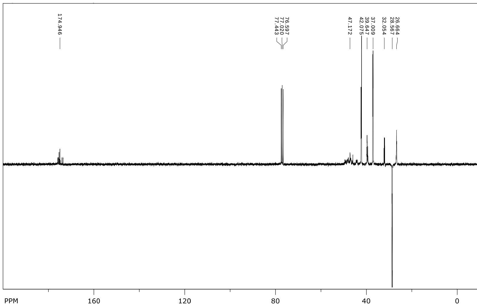
Figure S12. 13 C NMR (75 MHz, CDCl 3 ) spectrum of compound 6 .
