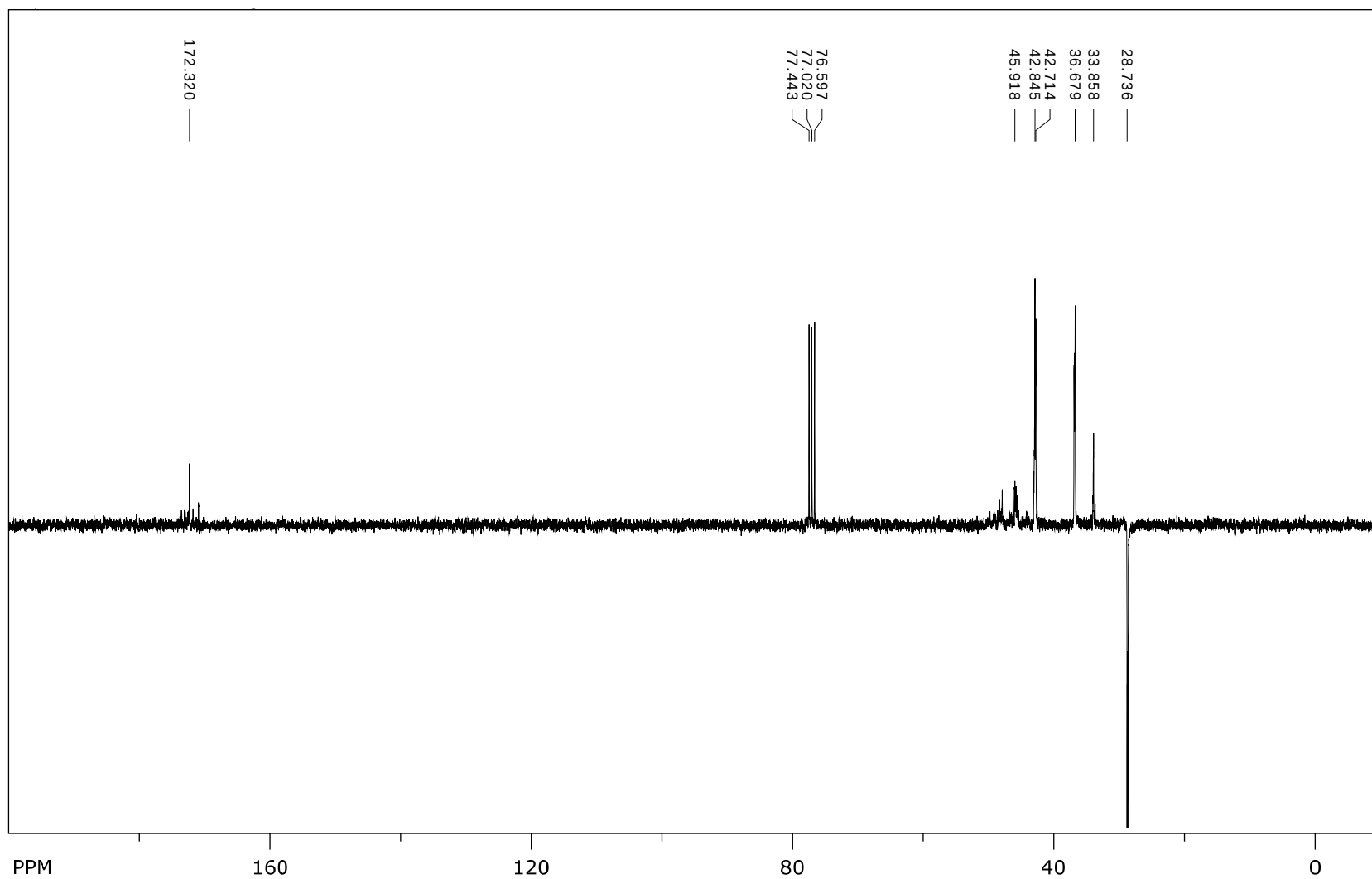
Figure S10. 13 C NMR (75 MHz, CDCl 3 ) spectrum of compound 5.
