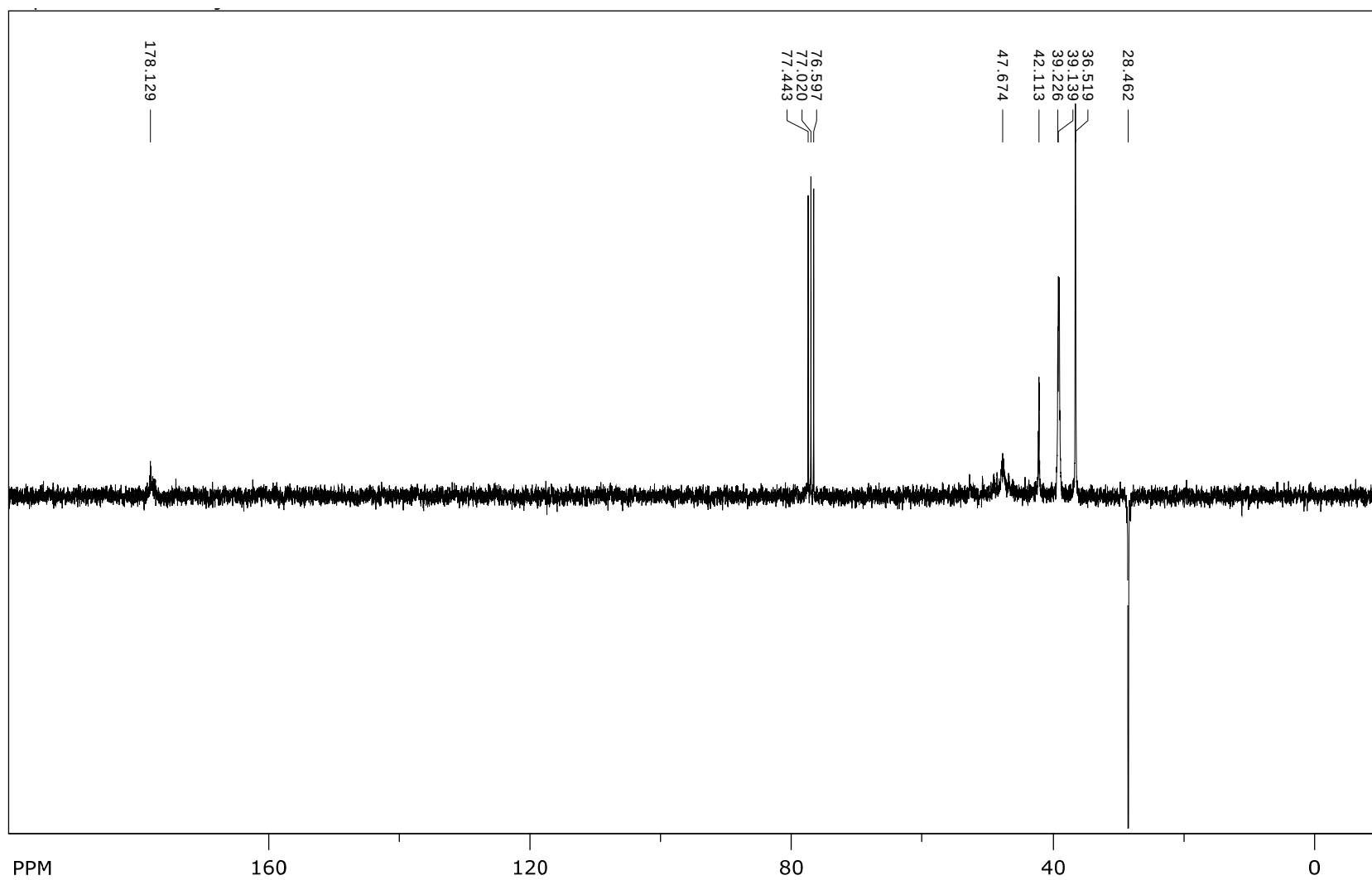
Figure S8. 13 C NMR (75 MHz, CDCl 3 ) spectrum of compound 4.
