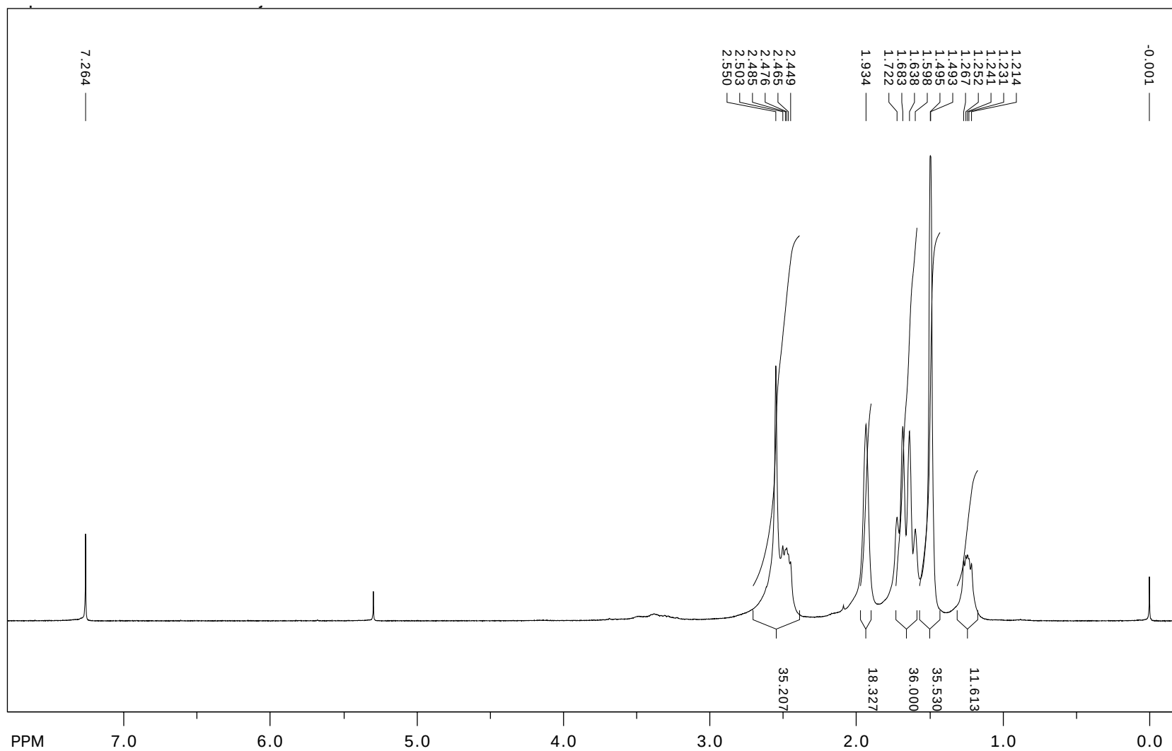
Figure S3. 1 H NMR (300 MHz, CDCl 3 ) spectrum of compound 2 .
