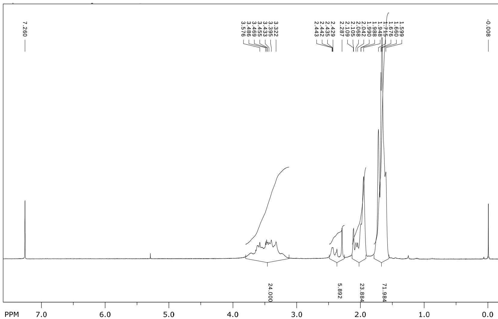
Figure S9. 1 H NMR (300 MHz, CDCl 3 ) spectrum of compound 5 .
