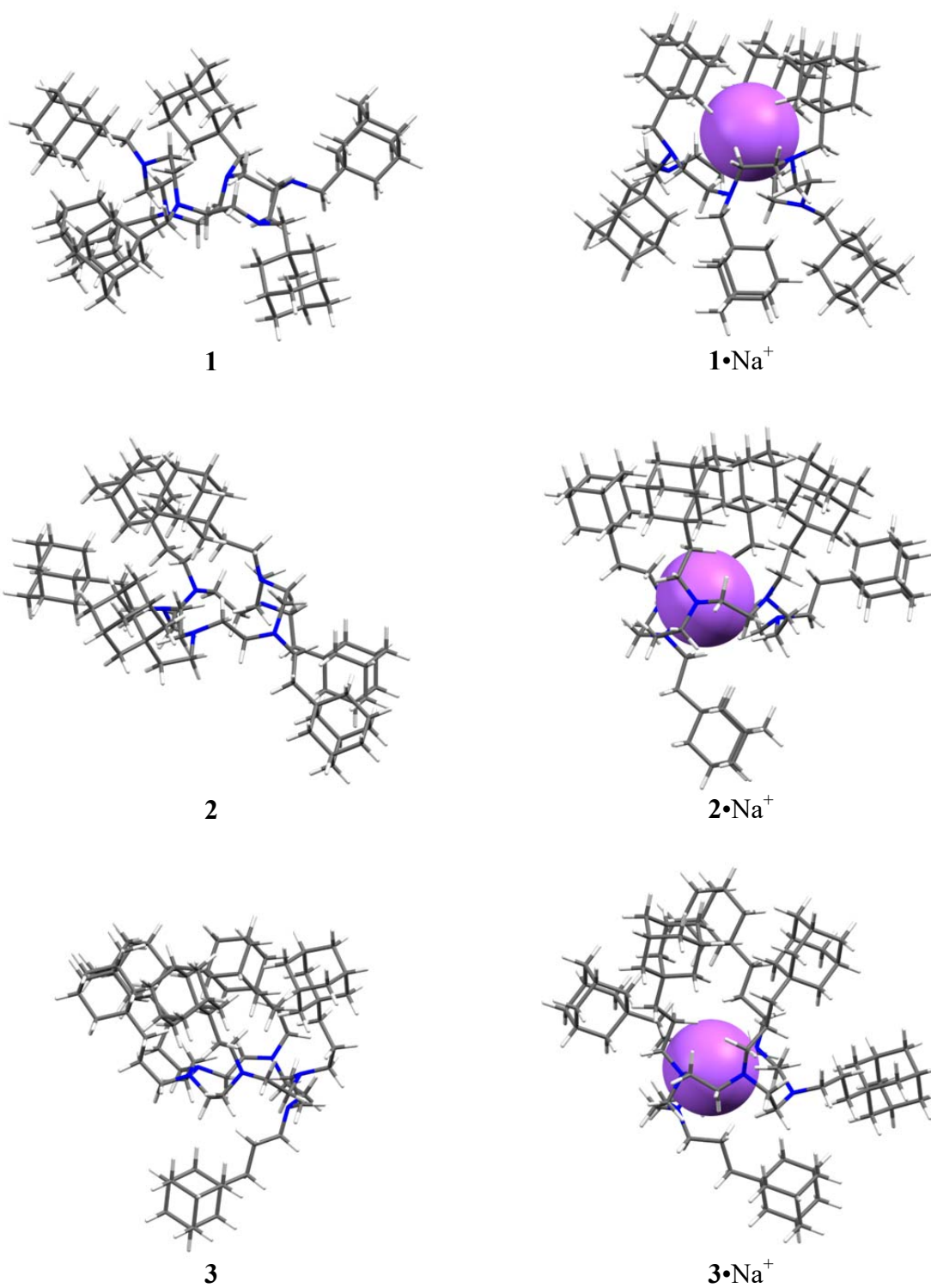
Figure S13. Optimized structures of compounds 1–3 (left) and their Na + complexes (right) computed at the r 2 SCAN-3c level of theory.
