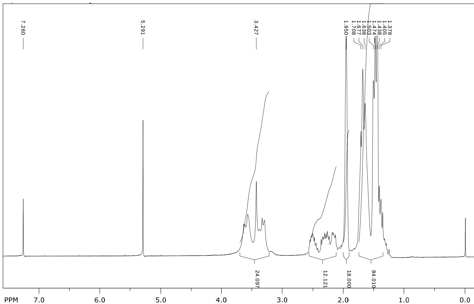
Figure S11. 1 H NMR (300 MHz, CDCl 3 ) spectrum of compound 6 .
