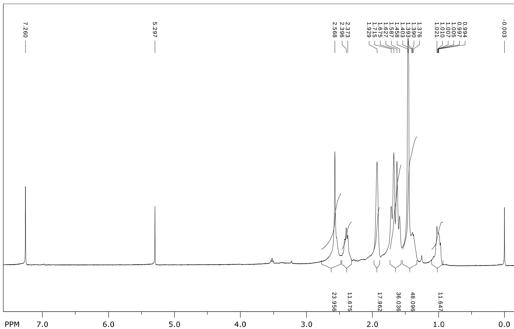
Figure S5. ^1\text{H} NMR (300 MHz, \text{CDCl}_3 ) spectrum of compound 3 .
