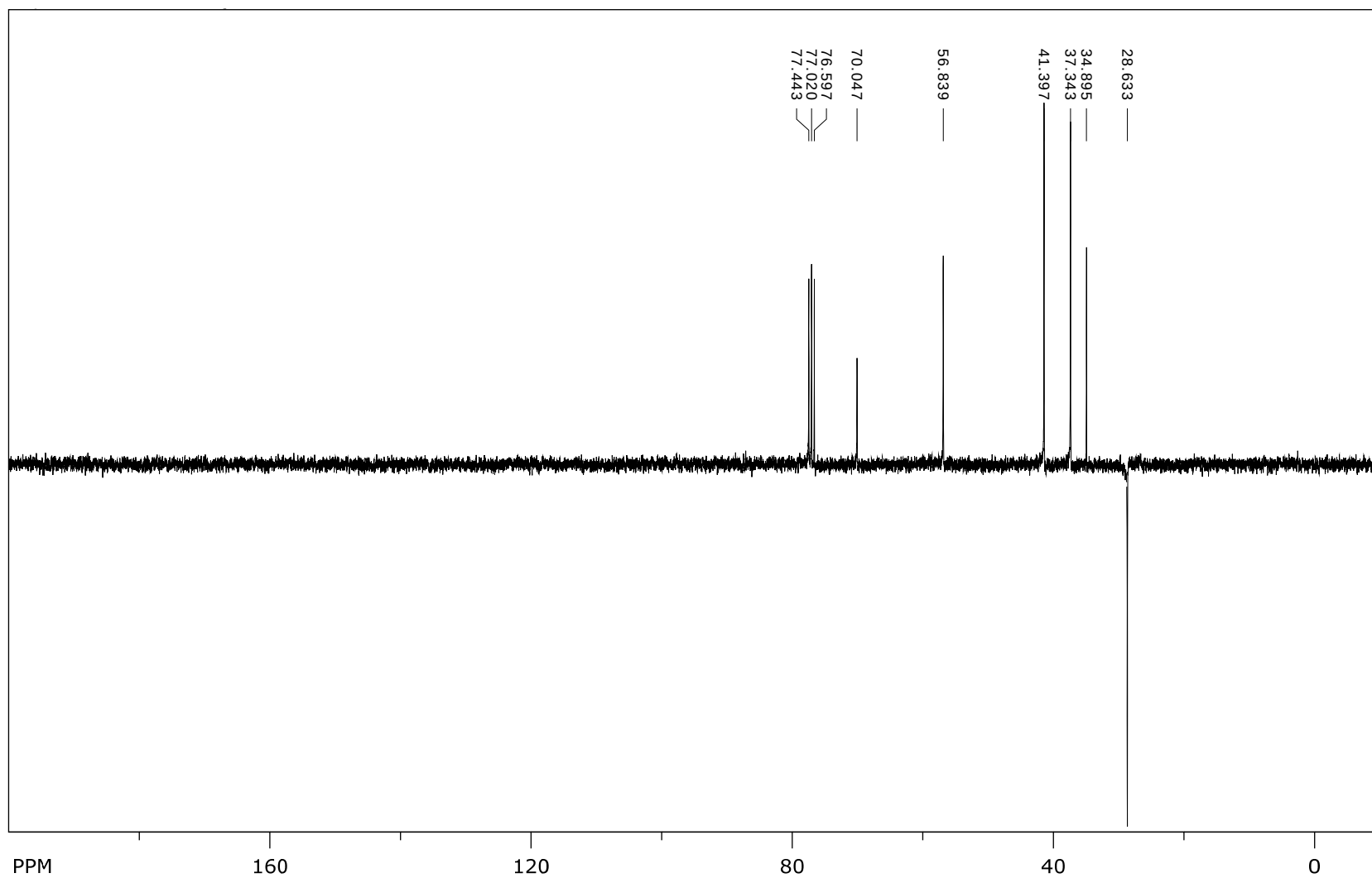
Figure S2. 13 C NMR (75 MHz, CDCl 3 ) spectrum of compound 1 .
