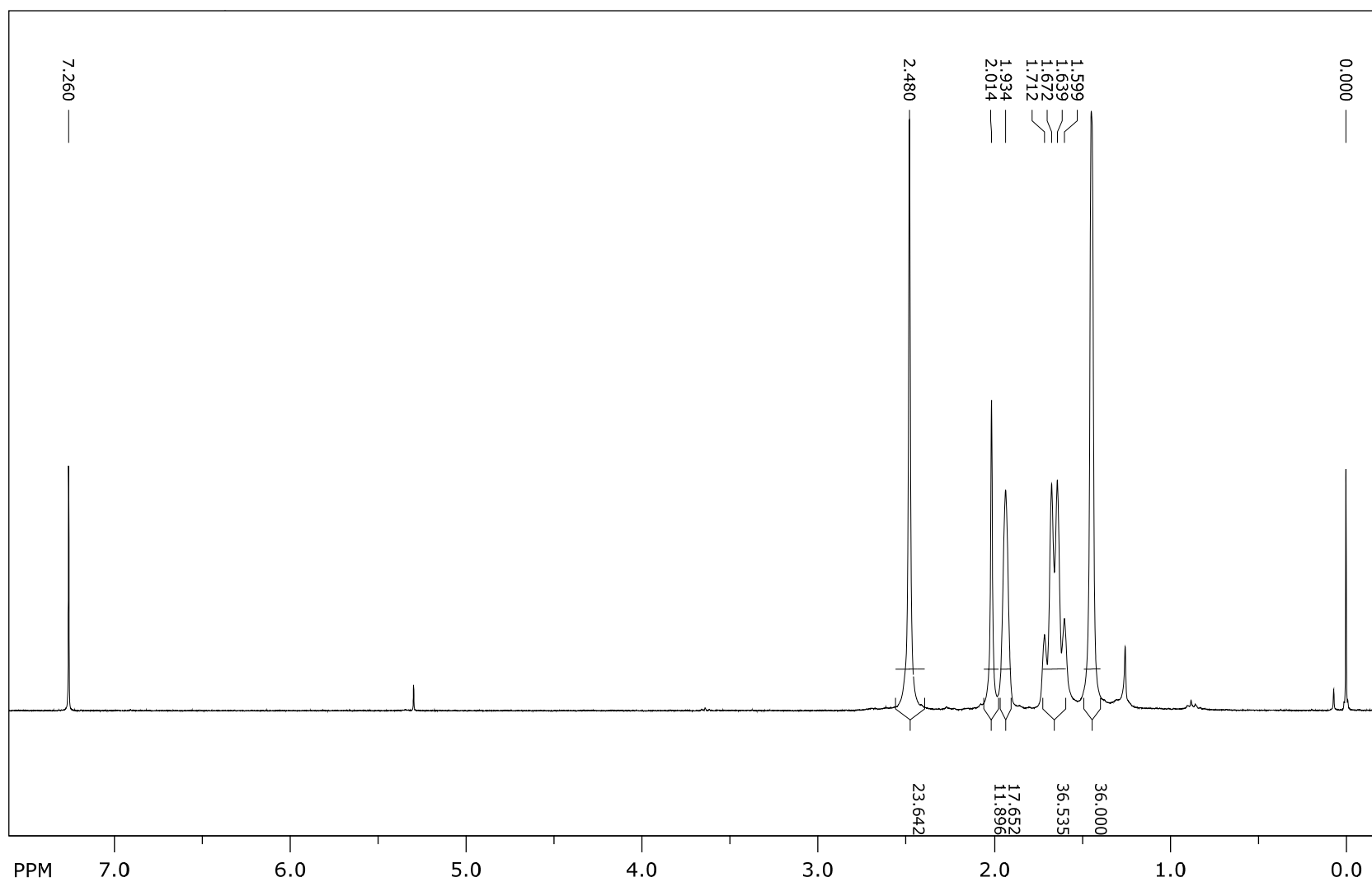
Figure S1. 1 H NMR (300 MHz, CDCl 3 ) spectrum of compound 1 .
