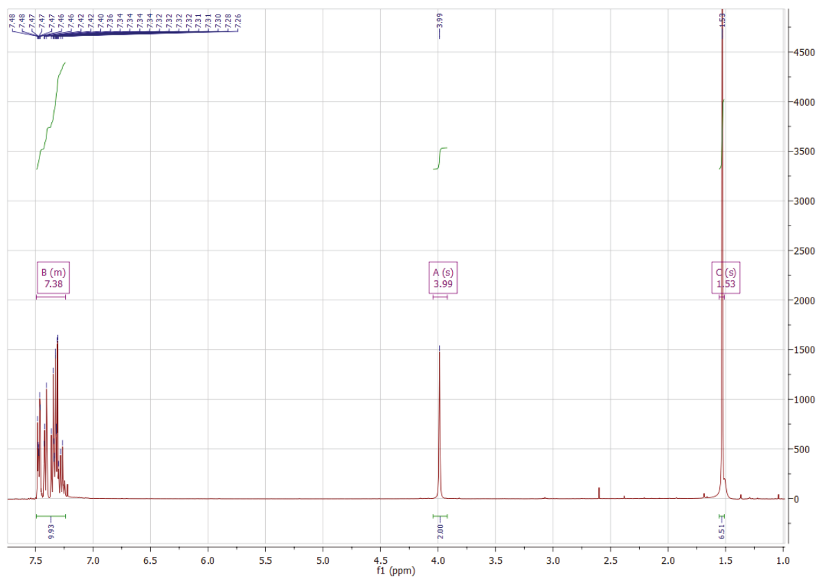
Figure 1. 1 H NMR spectrum of 1 in CDCl 3 .
