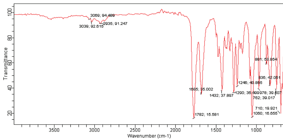
Figure 6. IR spectrum of 2-oxazolidone 2 .
