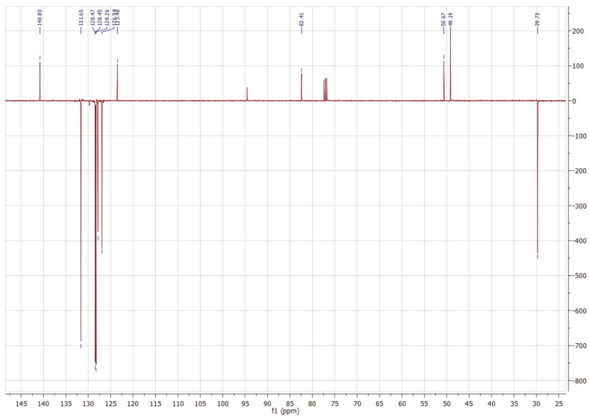
Figure 2. 13 C NMR spectrum of 1 in CDCl 3 .
