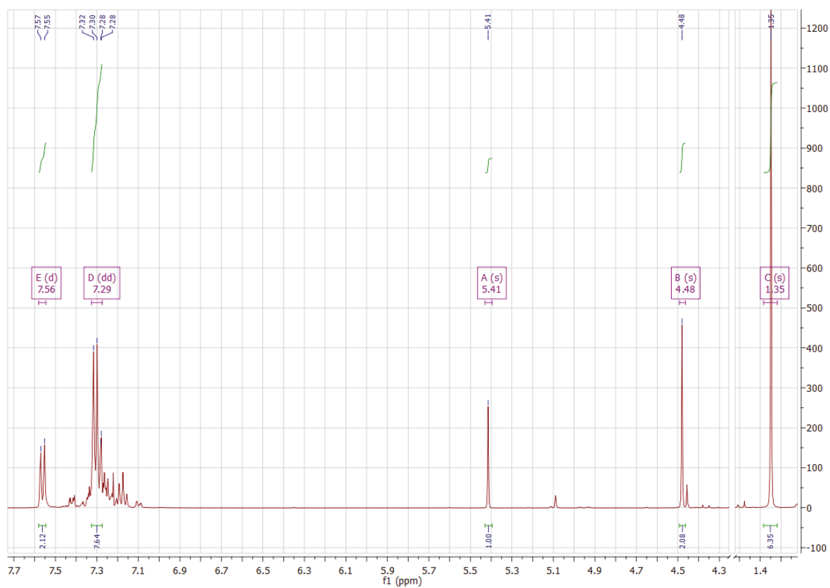
Figure 3. 1 H NMR spectrum of 2 in CDCl 3 .
