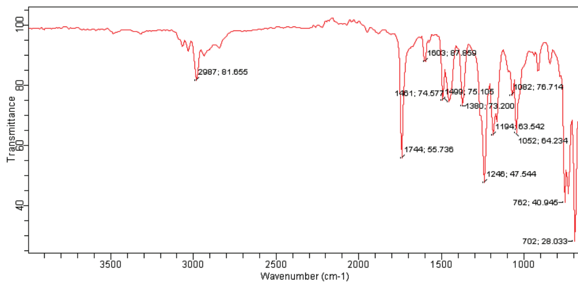
Figure 5. IR spectrum of 1 .
