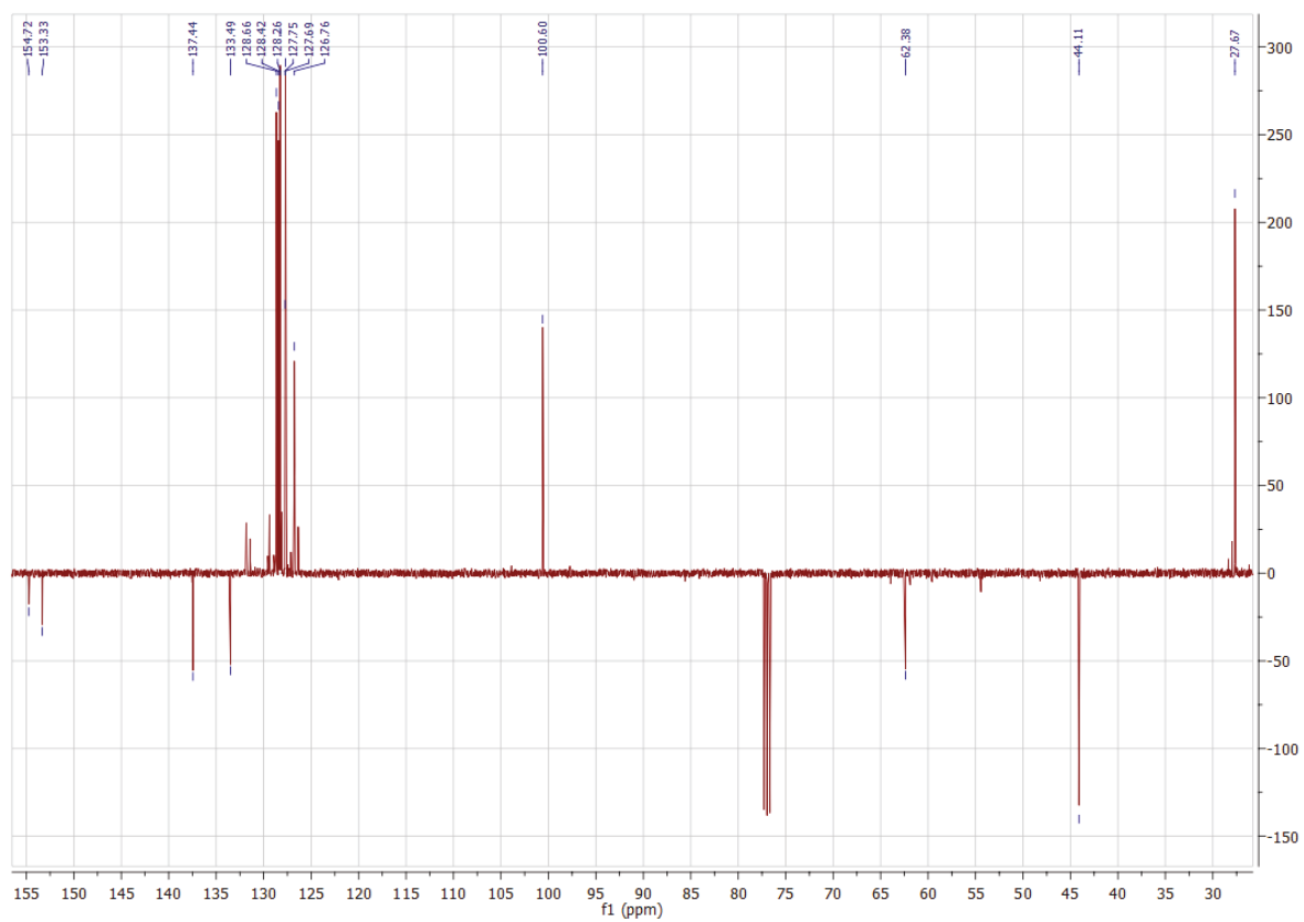
Figure 4. 13 C NMR spectrum of 2 in CDCl 3 .
