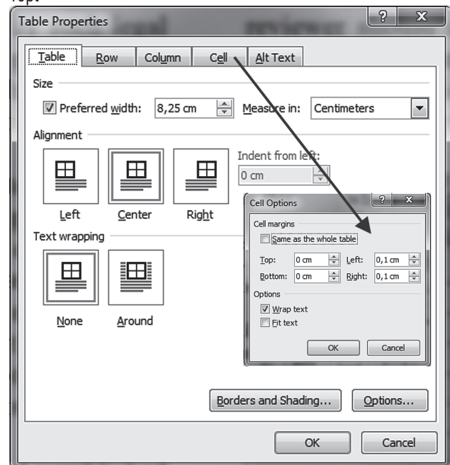
Figure 6 Table properties
